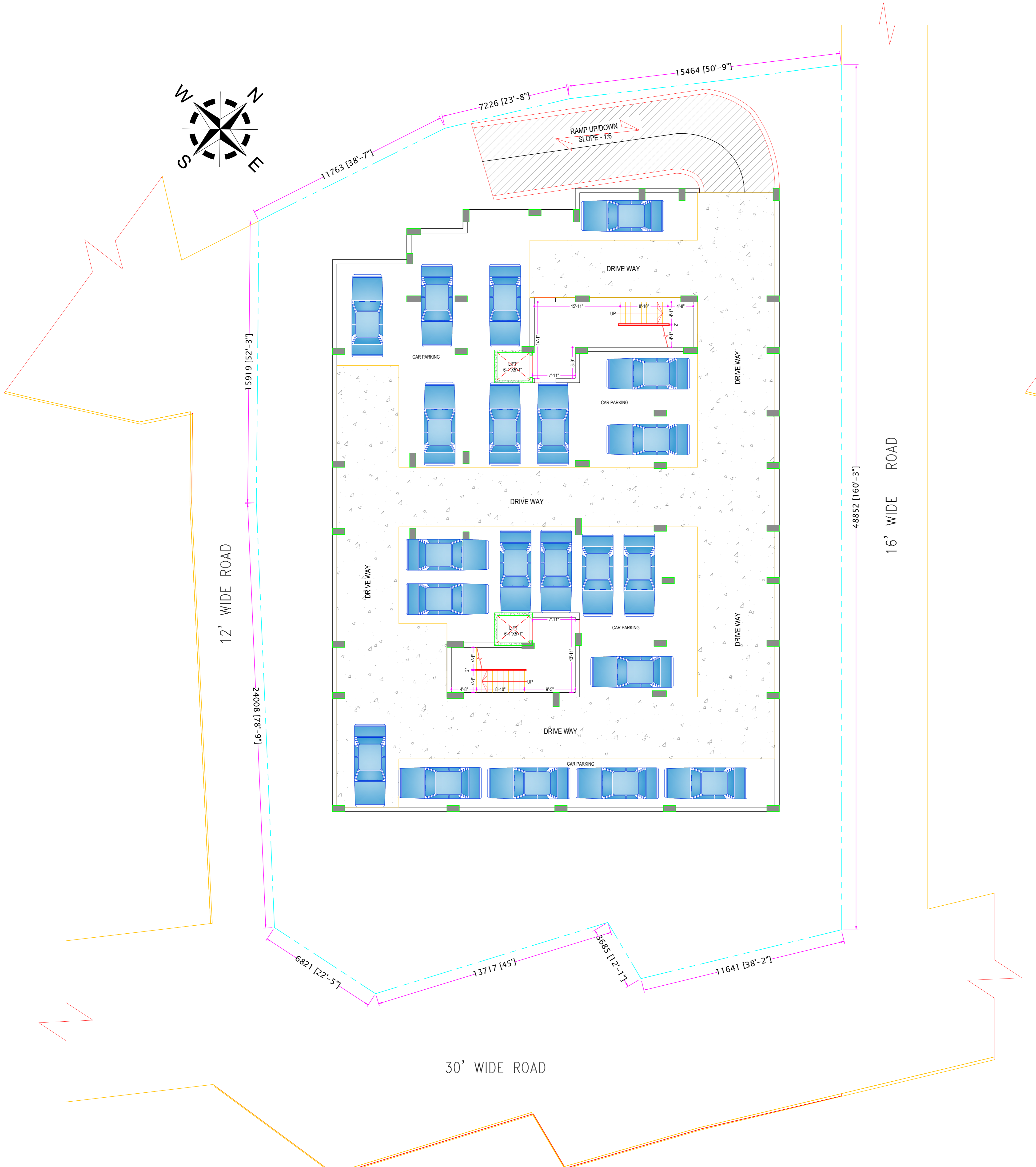
BASMENT FLOOR PLAN SCALE-1:100
